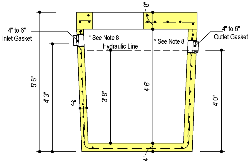
SECTION VIEW
