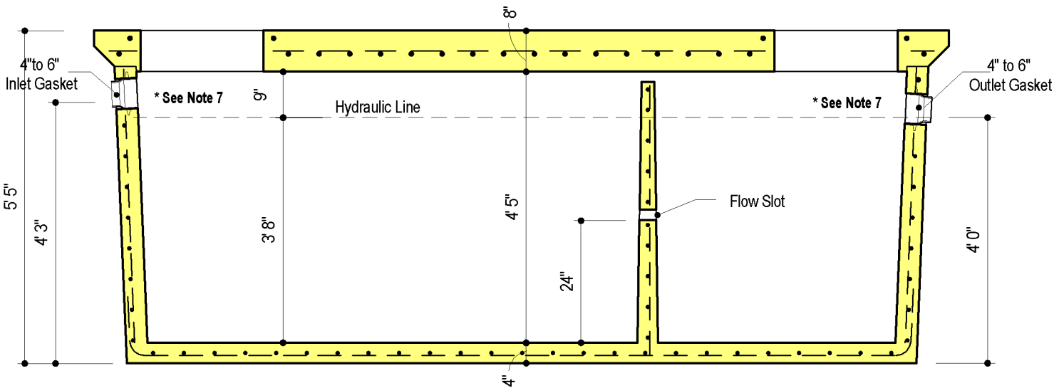
SECTION VIEW
